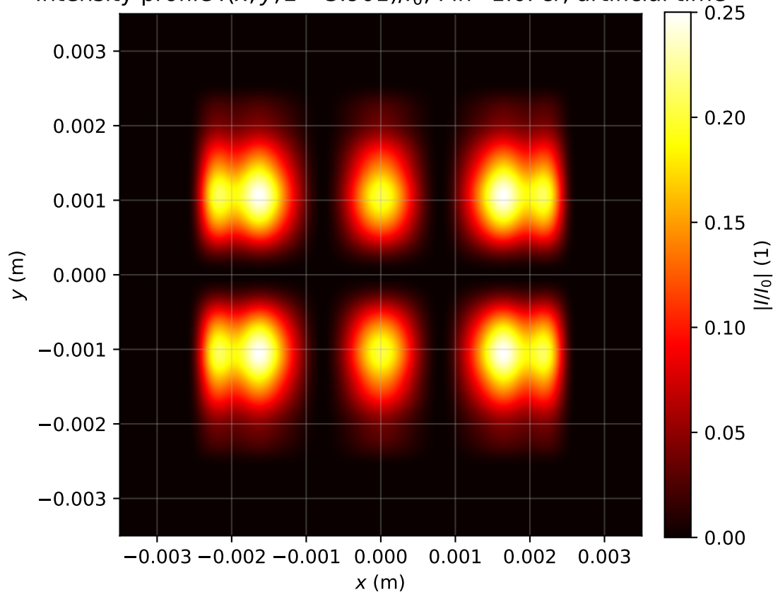
Intensity profile I(x, y, z = 3.901)/I_0 , P_{in}=1.0P_{cr} , artificial time
